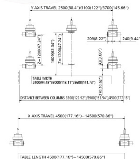
MACHINING RANGE OF KMC-G SERIES
